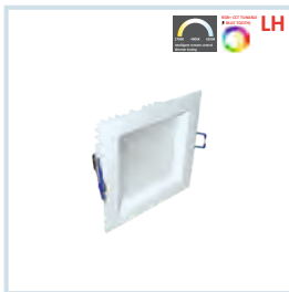
HLR-2982 (10W) Size : 110x110mmx36mm Cut-Out : 95x95mm
