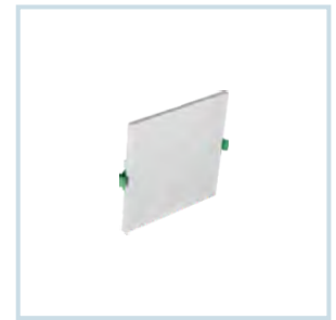
EB-9617 (8W) Size : 95x95x19mm Cut-Out : 85x85mm
