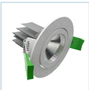
EB-9323 (10W) Size : Ø90x65mm Cut-Out : Ø85mm
