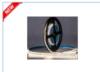
NEW HLL-4519 - 24V (White PCB - 8mm) 192 LED/MTR - 2835 - 20W Colour : TUNABLE (2700K-6500K)
