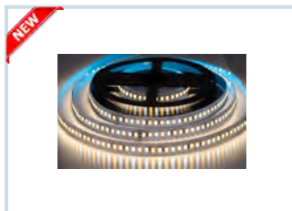
NEW HLL-4518 - 24V (White PCB - 8mm) 120 LED/MTR - 2835 - 10W Colour : TUNABLE (2700K-6500K)
