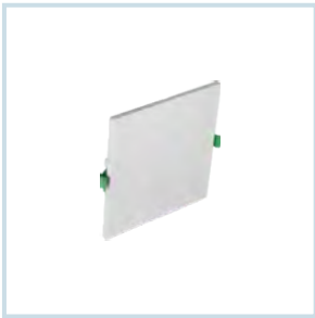
EB-9619 (15W) Size : 153x153x19mm Cut-Out : 142x142mm
