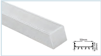
HLL-1013: SURFACE BODY - FULL SET STANDARD LENGTH : 2MTR SIZE : 50x18mm
