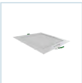
EB-9664(12W) Size : 170x170x12mm Cut-Out : 160x160mm
