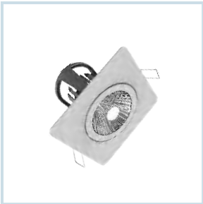
EB-9322 (6W) Size : 90x90x70mm Cut-Out : Ø80mm
