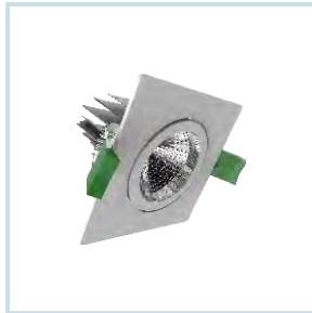
EB-9329 (10W) Size : 90x90x65mm Cut-Out : Ø85mm
